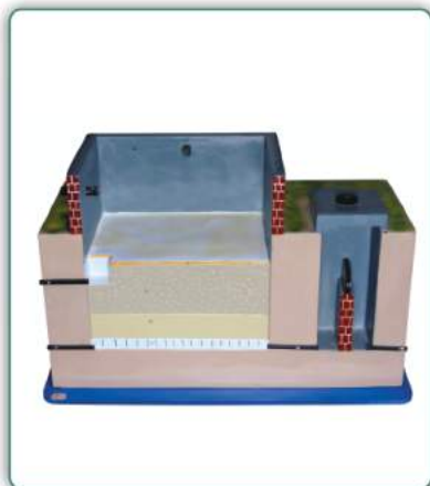
ZX 7107 - Slow Sand Filter
